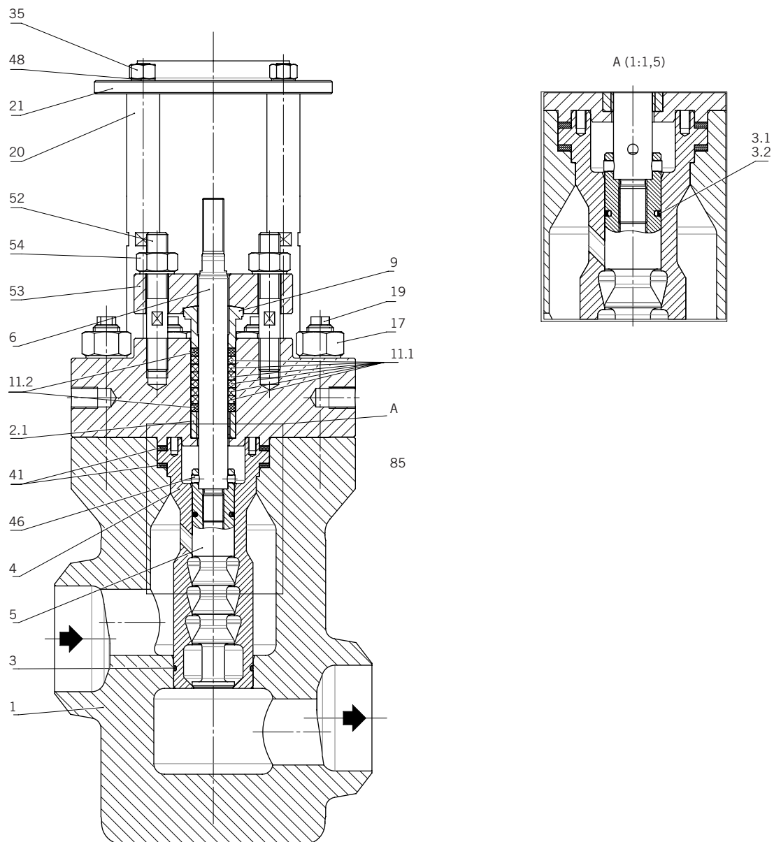
Sectional drawing (z-type)
