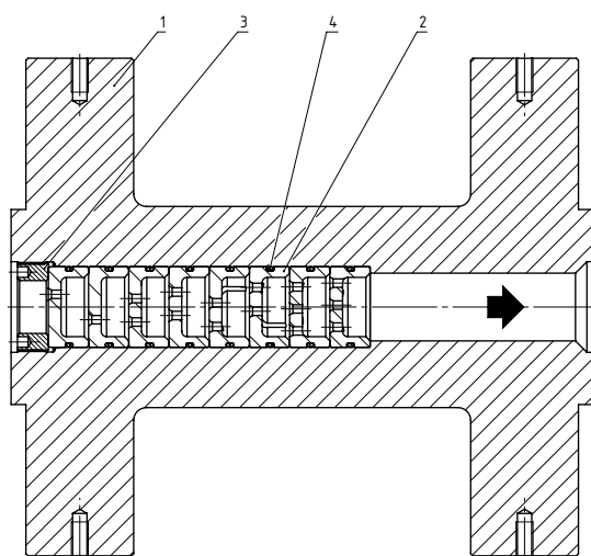
Sectional drawing (multi-stage)
